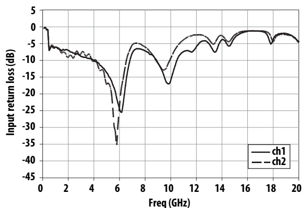
Figure 11. S11 vs Frequency and channel
